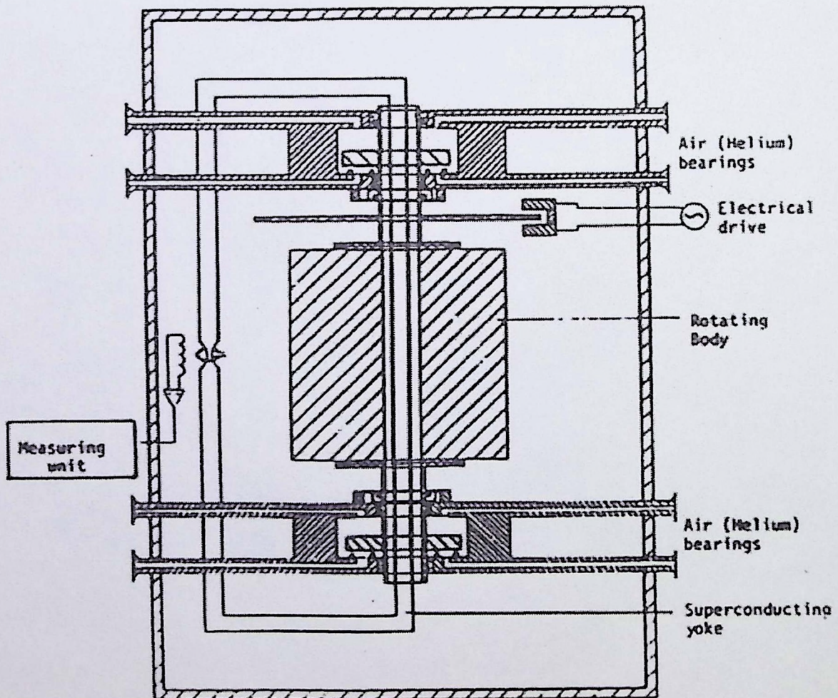
Fig. 6: Schematic diagram of the experimental set-up for the measurement of the weak magnetic field generated by a rotating crystal (Harasim et al 1985)
